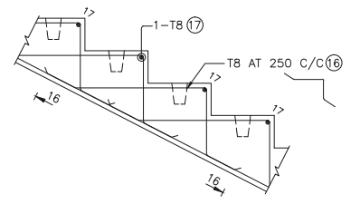
TYPICAL RC DETAIL OF STEP
